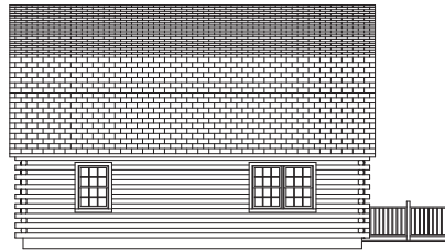
REAR ELEVATION
