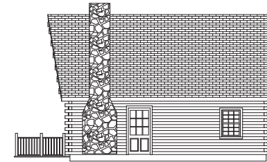
LEFT ELEVATION
