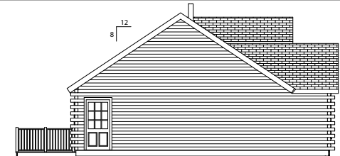
LEFT ELEVATION
