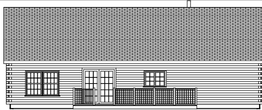
REAR ELEVATION
